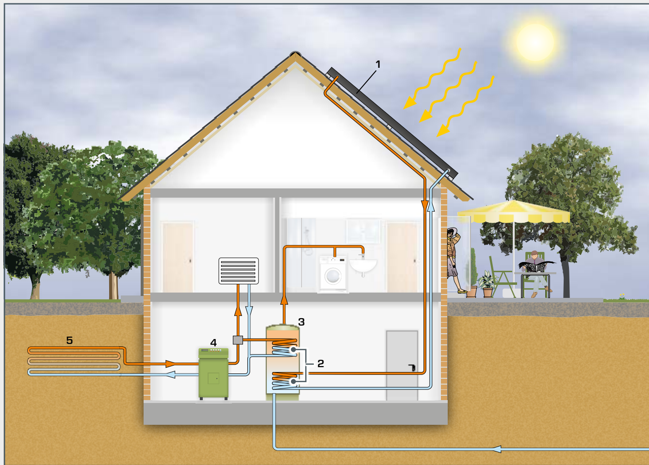
1 flat collector, 2 heat exchanger, 3 hot water storage tank, 4 heat pump, 5 geothermal energy absorber; ■ hot heat transfer fluid, ■ cold heat transfer fluid, ■ reffridgerant, high pressure, ■ reffridgerant, low pressure
